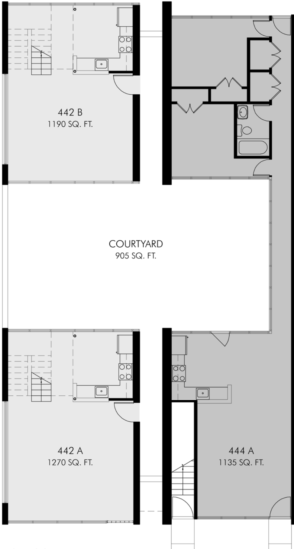
FIRST FLOOR
